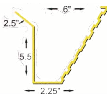
7 1/4" Tile Gutter Decco Face
